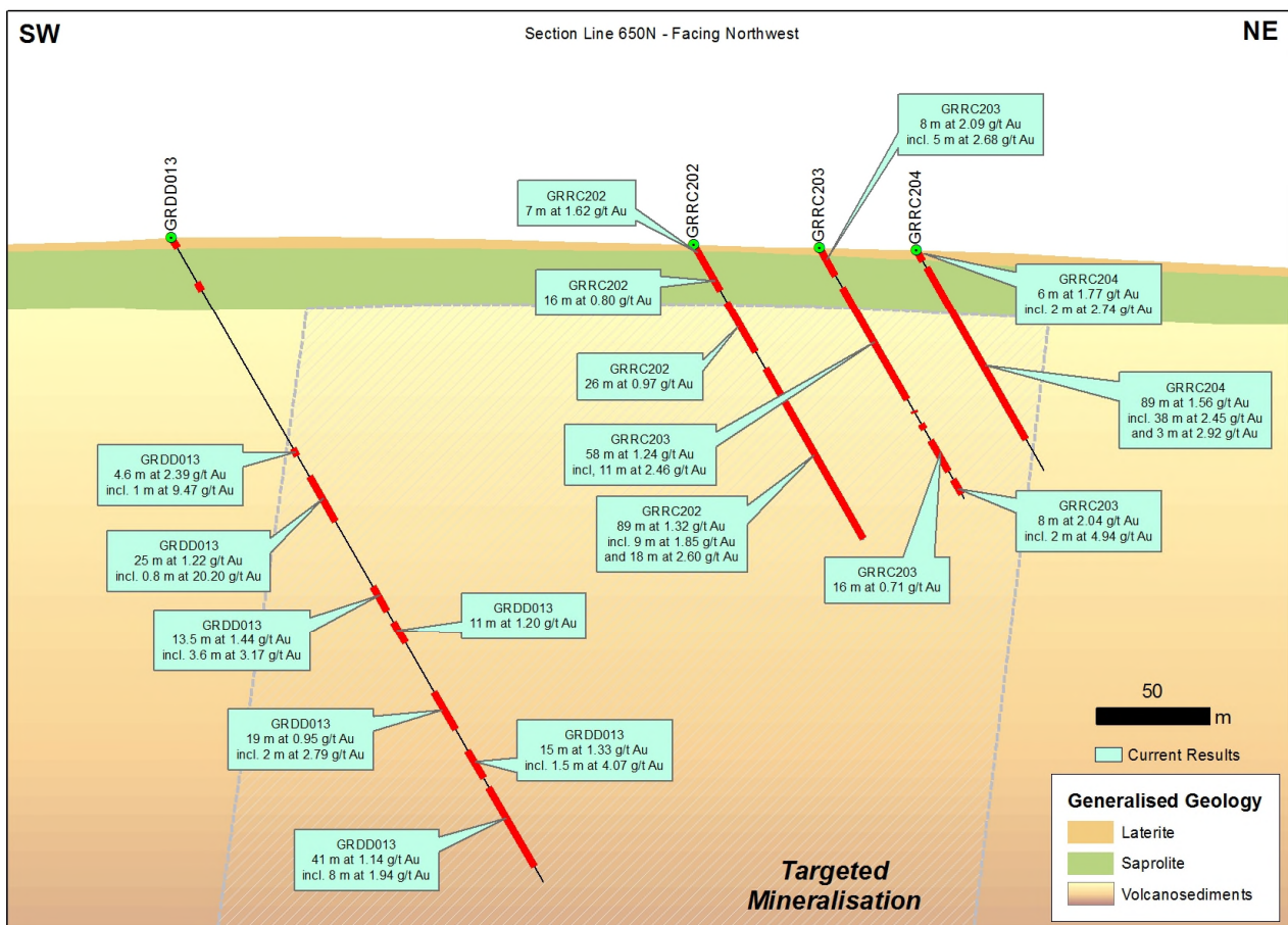
Figure 2: Section across Line 650N showing the main mineralised intercepts
