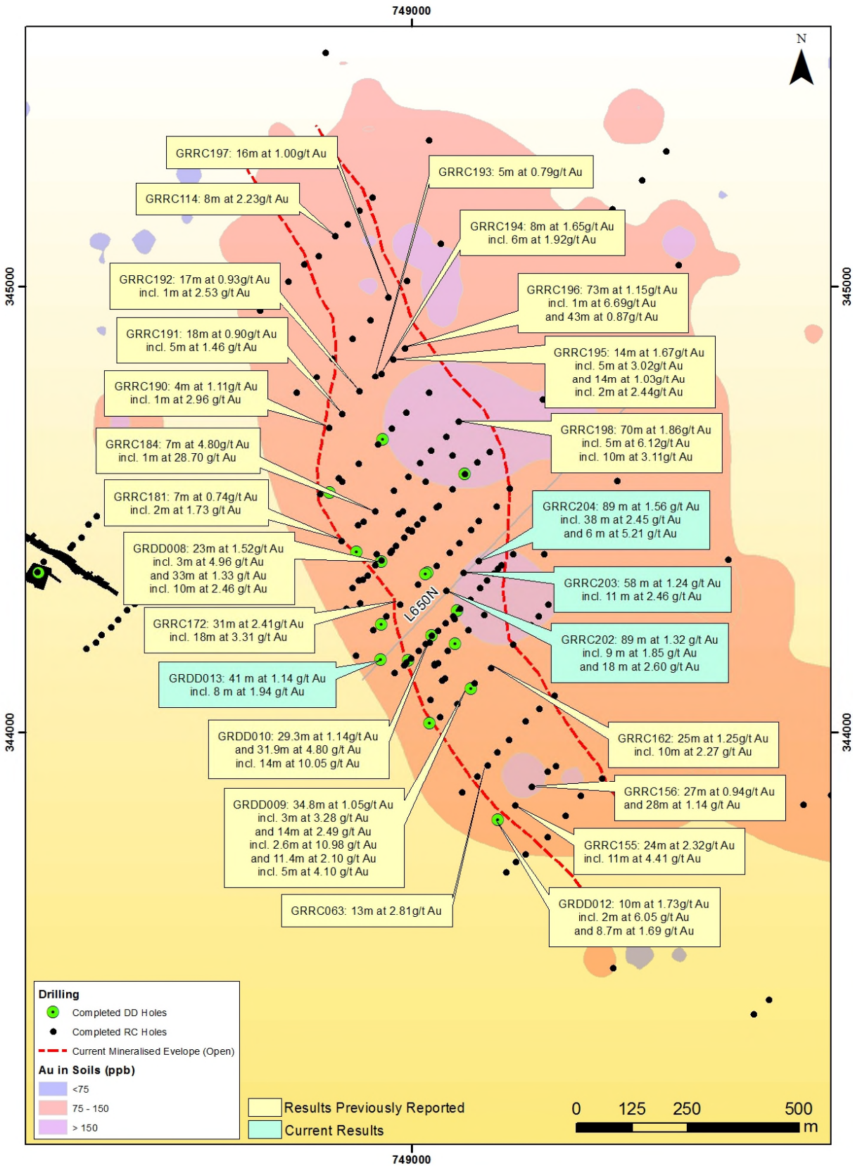
Figure 1: RC drill hole locations and significant mineralised intercepts at Kebigada.
